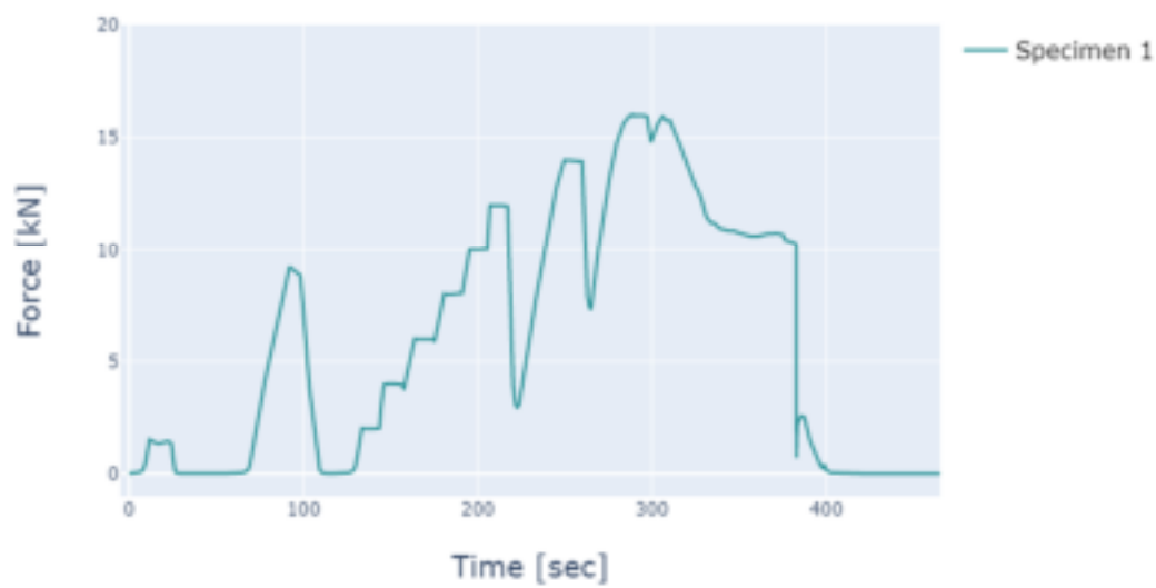
Appendix Figure B-1. Ecoply specimen 1 force results
