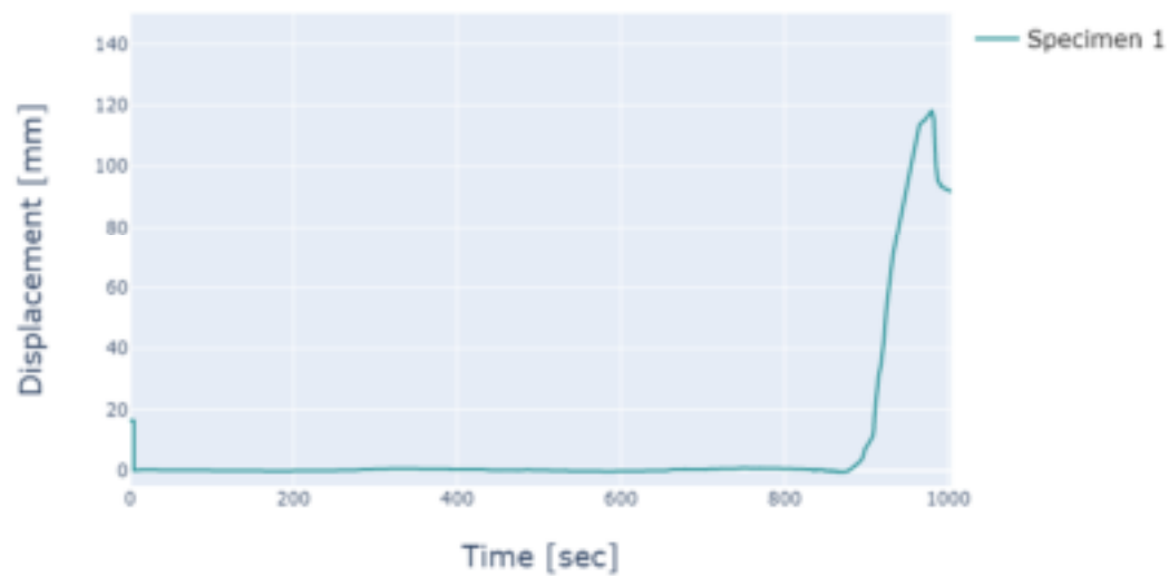
Appendix Figure C-7. ST900 Specimen 1 midspan PIR-substrate relative displacement results
