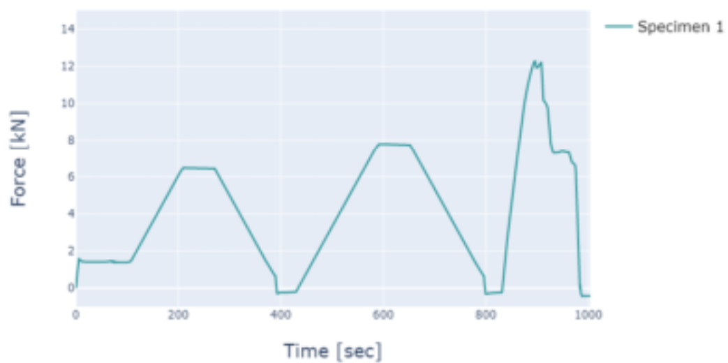
Appendix Figure C-1. ST900 specimen 1 force results
