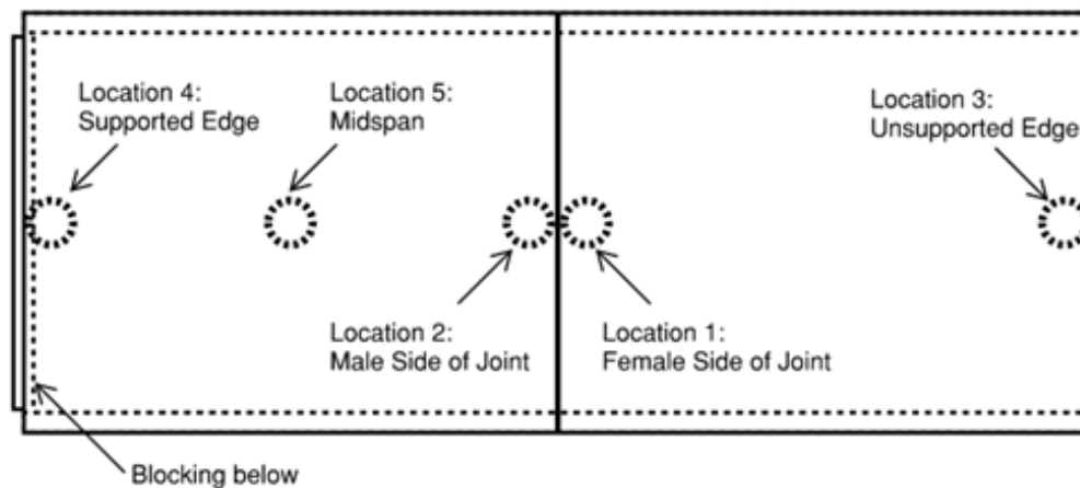
Figure 8-3. Point load application locations
