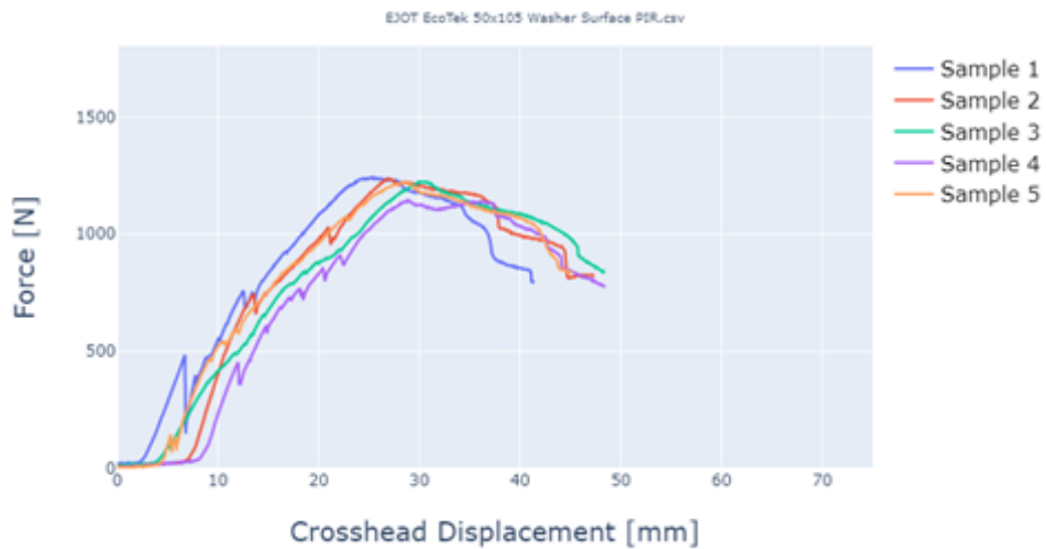
Figure 6-2. EcoTek 50mm x 105 mm plastic washer pull-through force-displacement results
