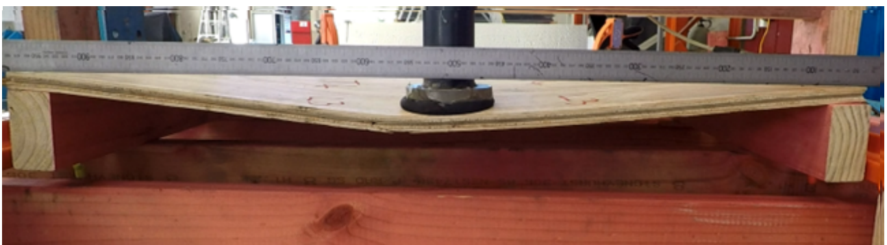
Figure 8-10. Deflection under ULS load (Location 3, Sample 2)
