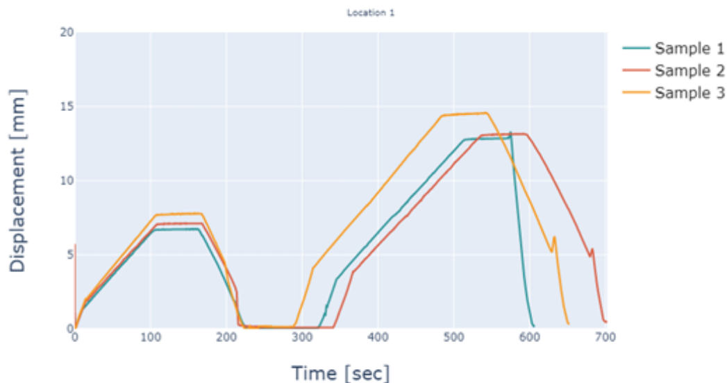
Figure 8-9. Location 1 (female side of joint) displacement results
