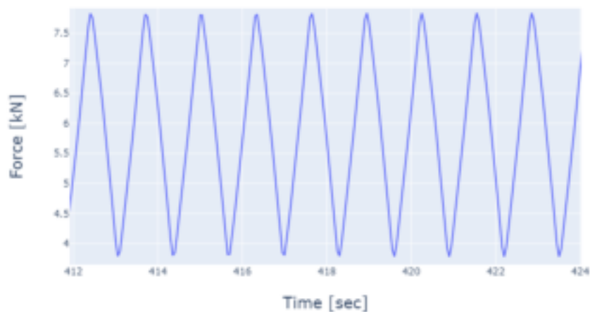
Figure 9-13. Cyclic loading protocol at approximately 0.75 Hz
