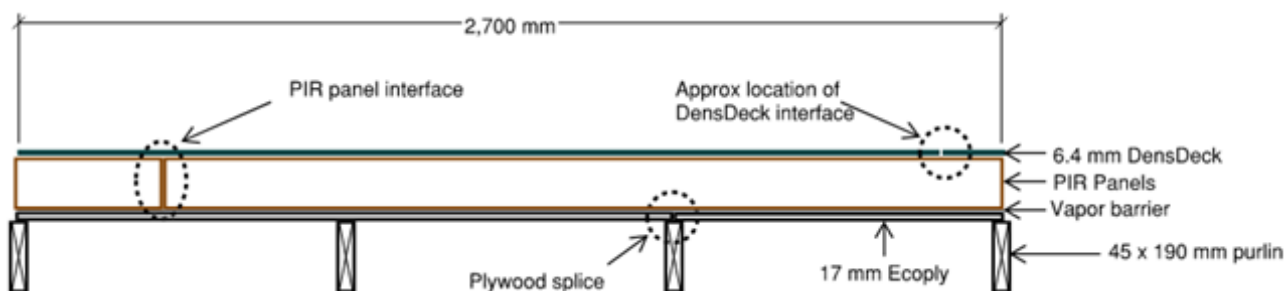
Figure 9-6. Viking Roofspec roof build up on timber subframe
