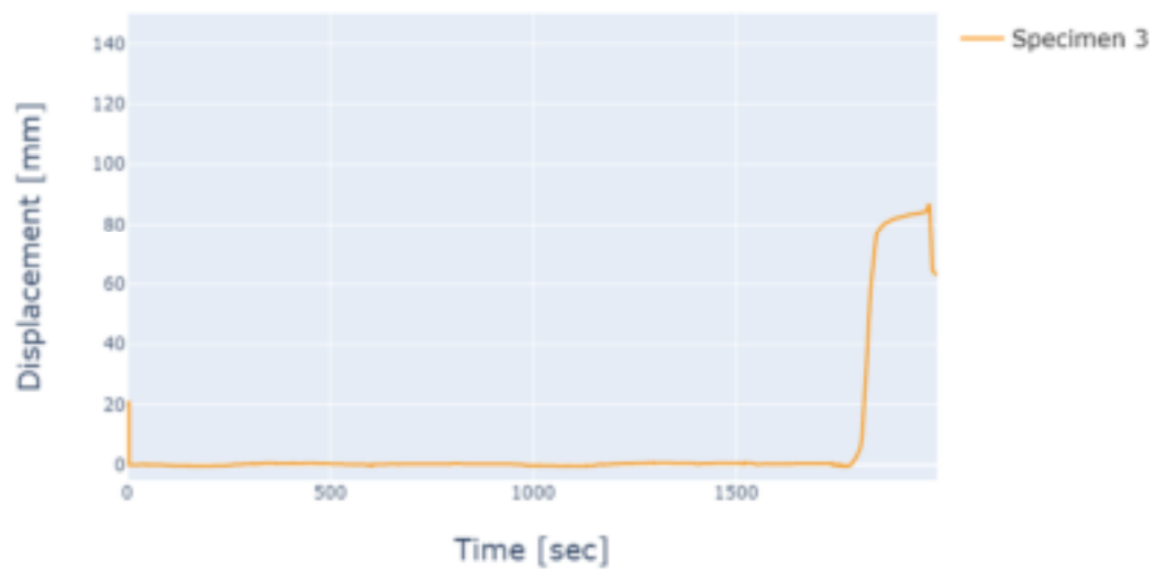
Appendix Figure C-9. ST900 Specimen 3 midspan PIR-substrate relative displacement results
