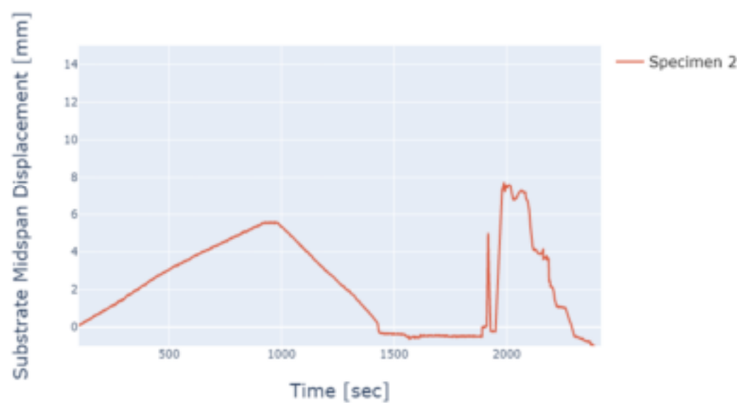
Appendix Figure B-5. Ecoply specimen 2 substrate midspan displacement results
