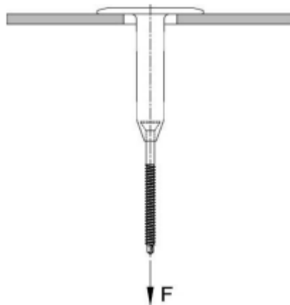
Figure 6-1. Principle of a plastic washer pull through test (EAD 030351-00-0402)
