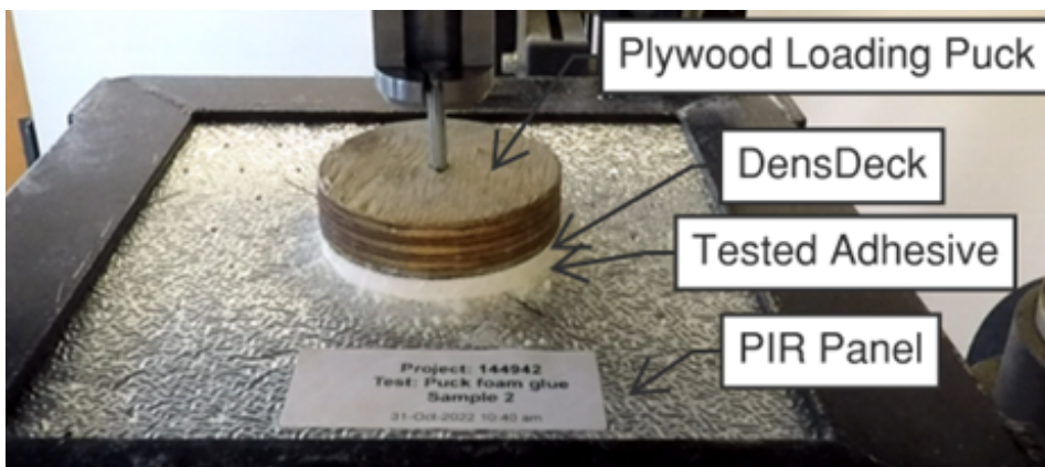
Figure 7-3. Viking Soudafoam adhesive sample
