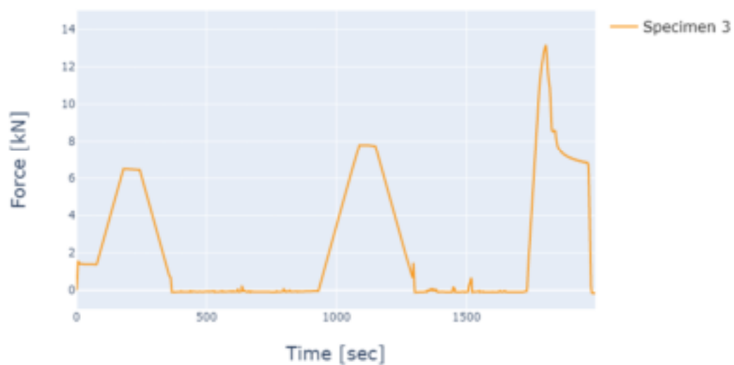
Appendix Figure C-3. ST900 specimen 3 force results
