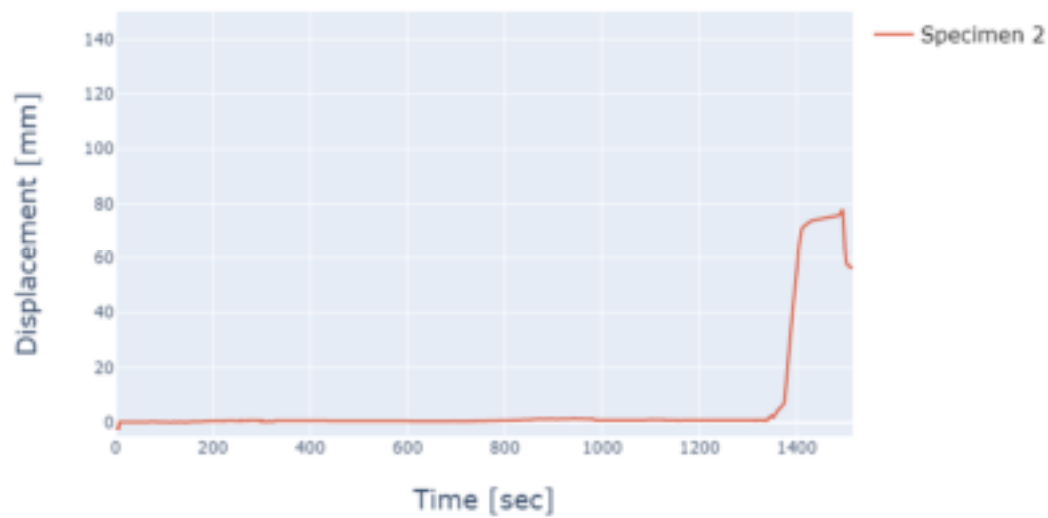
Figure 9-18. ST900 specimen 2 PIR-substrate relative midspan displacement results
