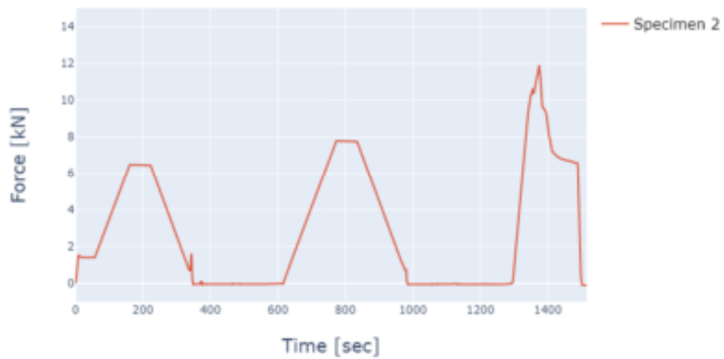
Figure 9-16. ST900 specimen 2 force results
