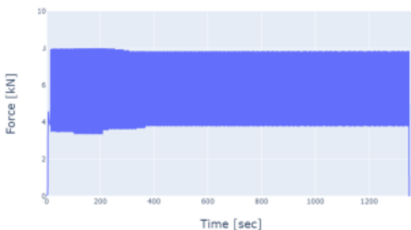
Figure 9-12. Example of the Cyclic Loading Protocol (40% to 80% Range)
