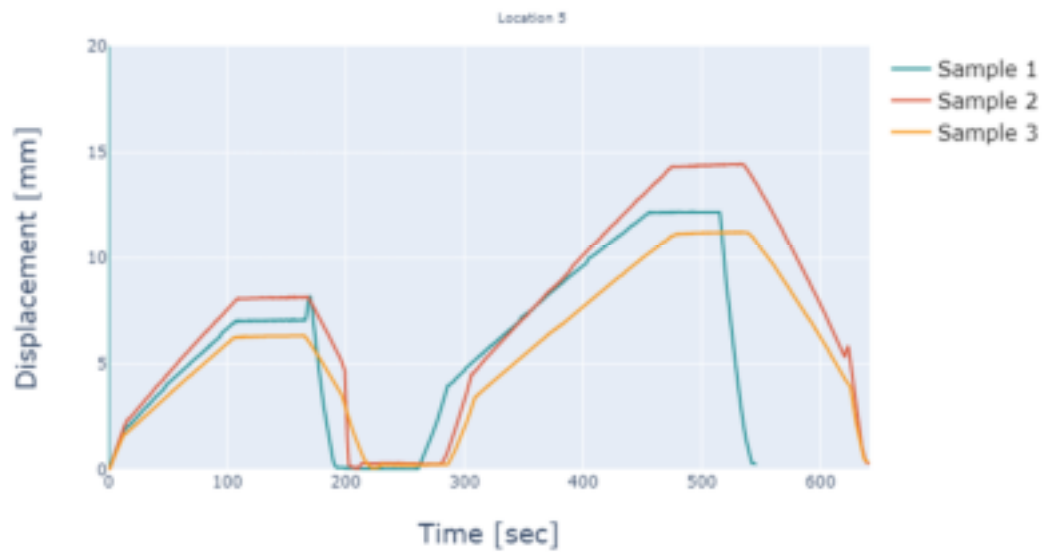
Appendix Figure A-3. Location 5 (midspan) displacement results
