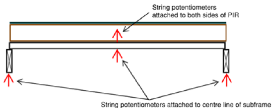
Figure 9-4. String potentiometer locations on ST900 subframe during SLS and Cyclic tests
