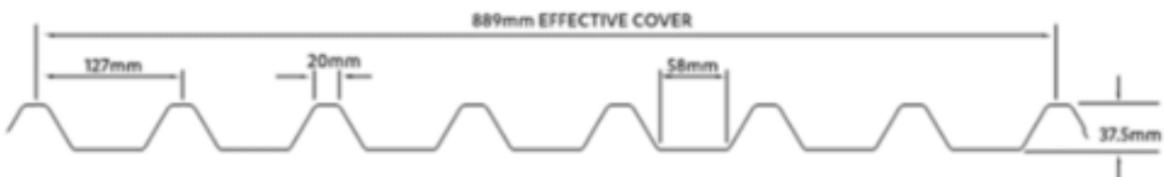
Figure 3-3. Alternative acceptable profile - Steel and Tube ST7 profile (shown opposite to installed orientation)
