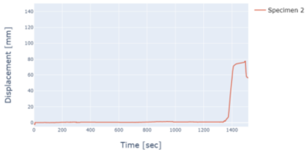
Appendix Figure C-8. ST900 Specimen 2 midspan PIR-substrate relative displacement results
