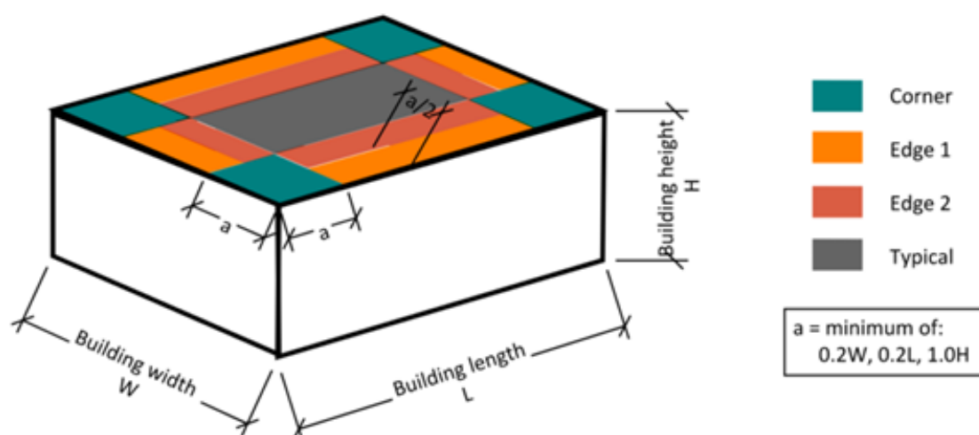
Figure 10-1. Roof regions for determination of fixing quantity
