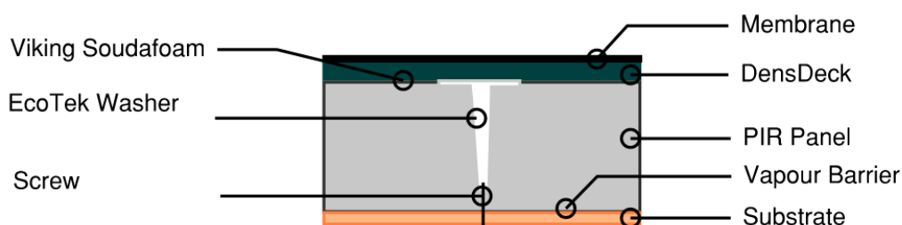
Figure 1-1. Viking RoofSpec Example Build Up
