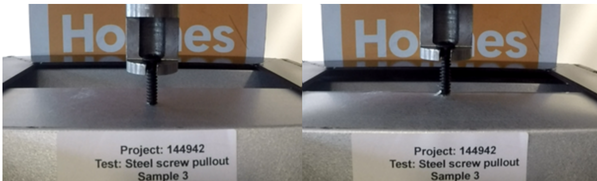
Figure 5-5. ST900 deforming under withdrawal load
