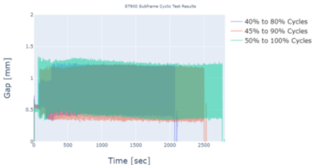
Figure 9-21. Cyclic test gap opening (ST900 subframe)
