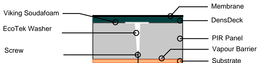
Figure 3-1. Example WarmRoof 2 construction.
