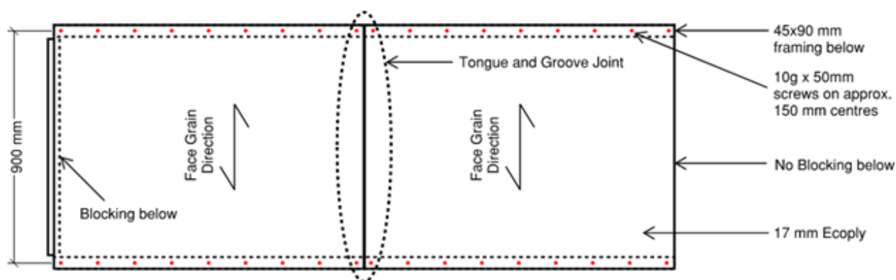
Figure 8-1. Plywood Point Load Testing Specimen
