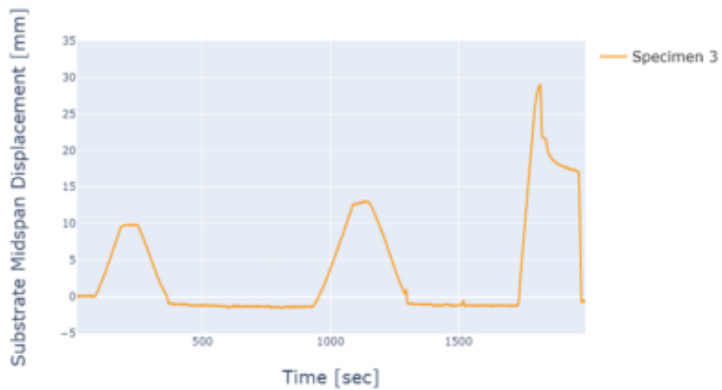
Appendix Figure C-6. ST900 specimen 3 substrate midspan displacement results
