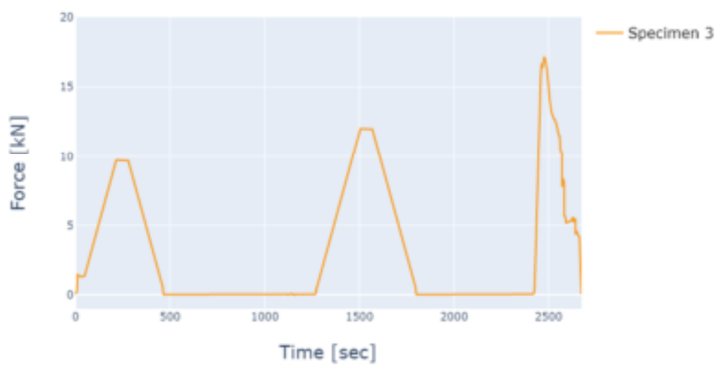
Appendix Figure B-3. Ecoply specimen 3 force results
