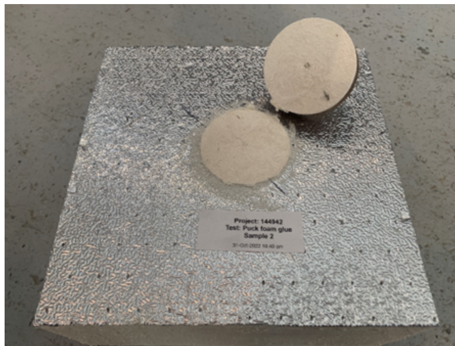
Figure 7-5. Delaminated DensDeck layer
