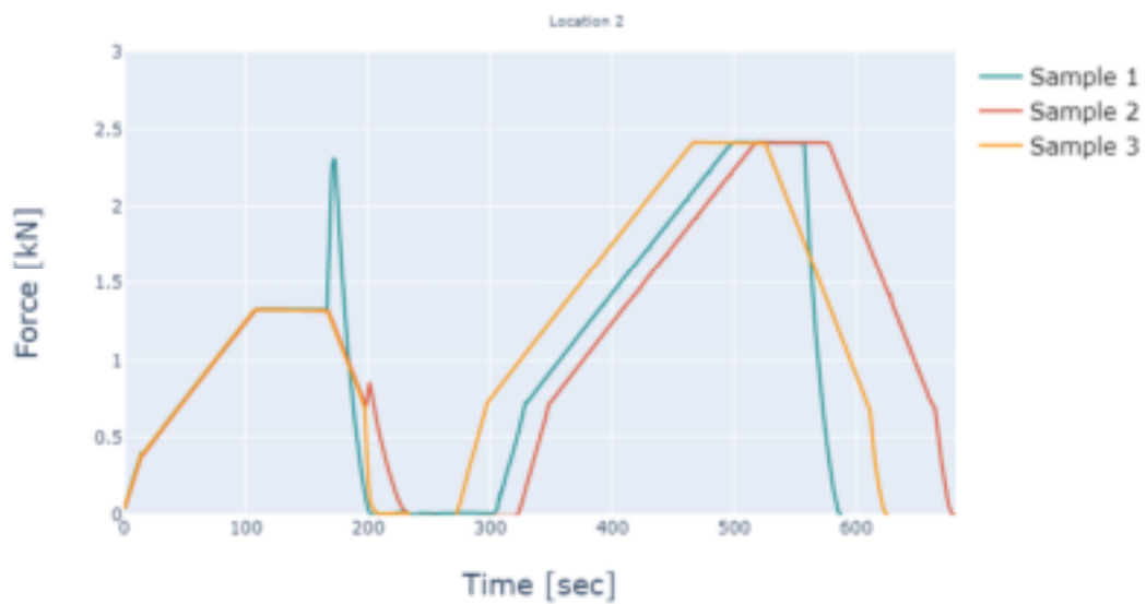
Appendix Figure A-4. Location 2 (male side of joint) force results
