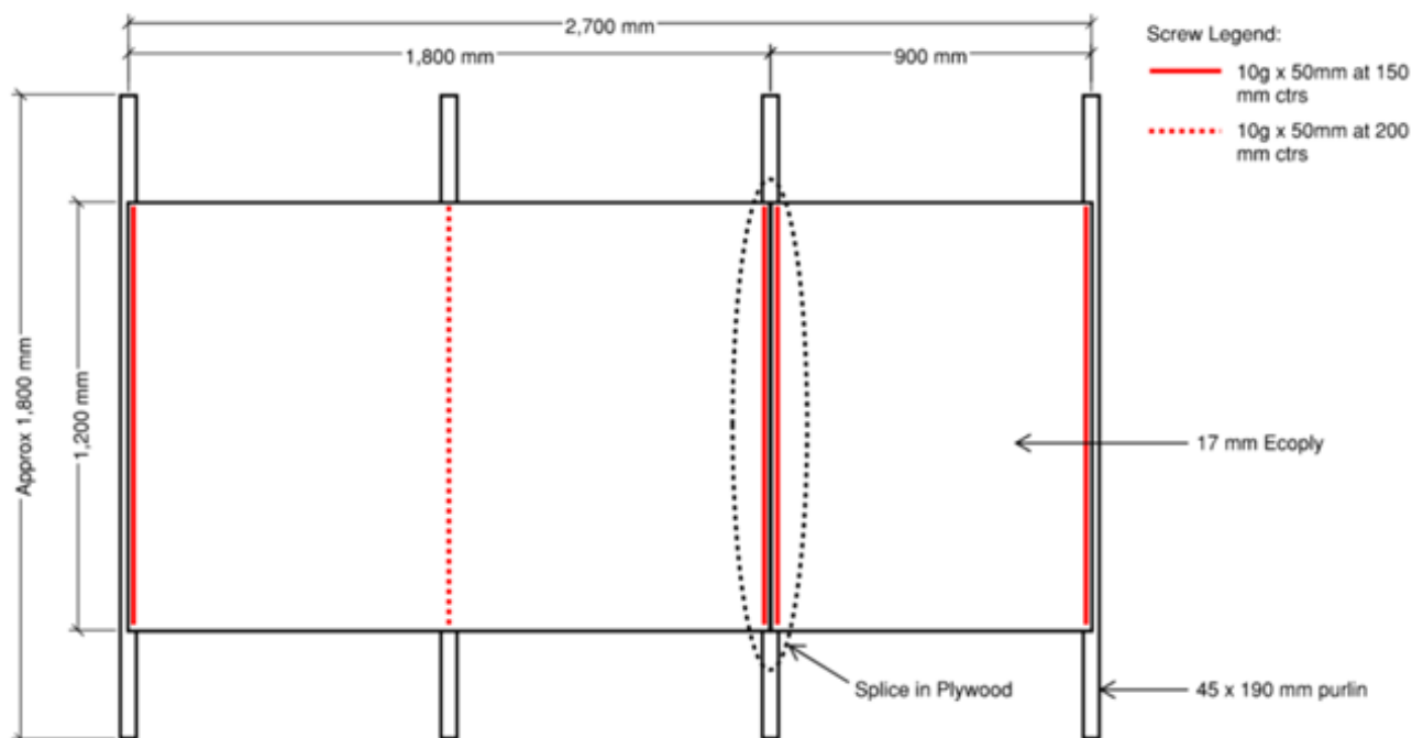
Figure 9-5. Plywood subframe drawing
