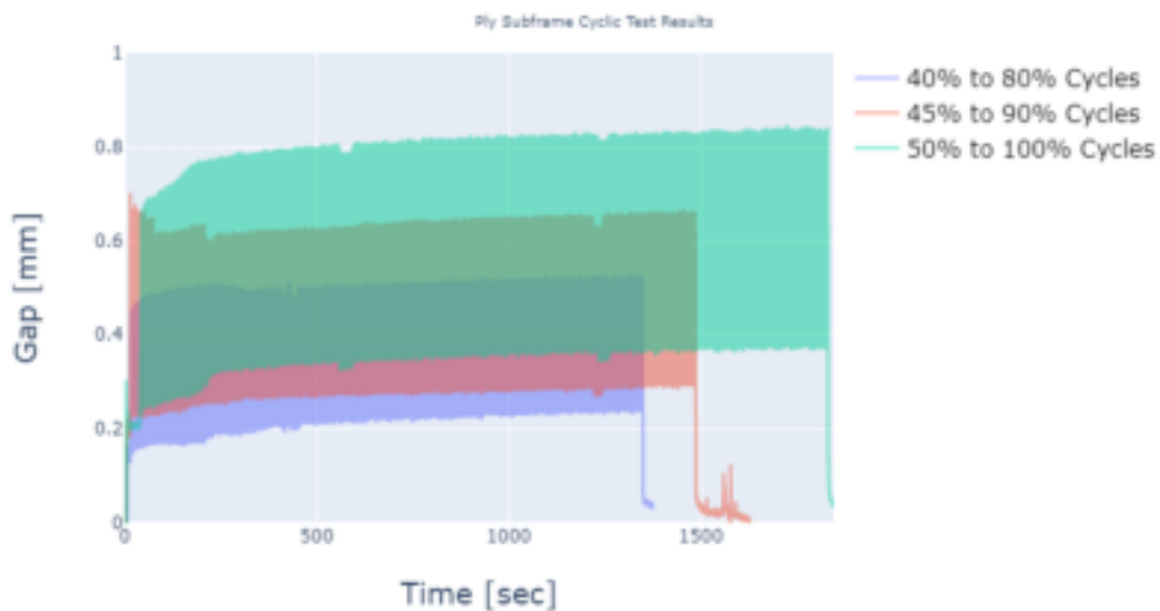
Figure 9-15. Cyclic test gap opening (plywood subframe)
