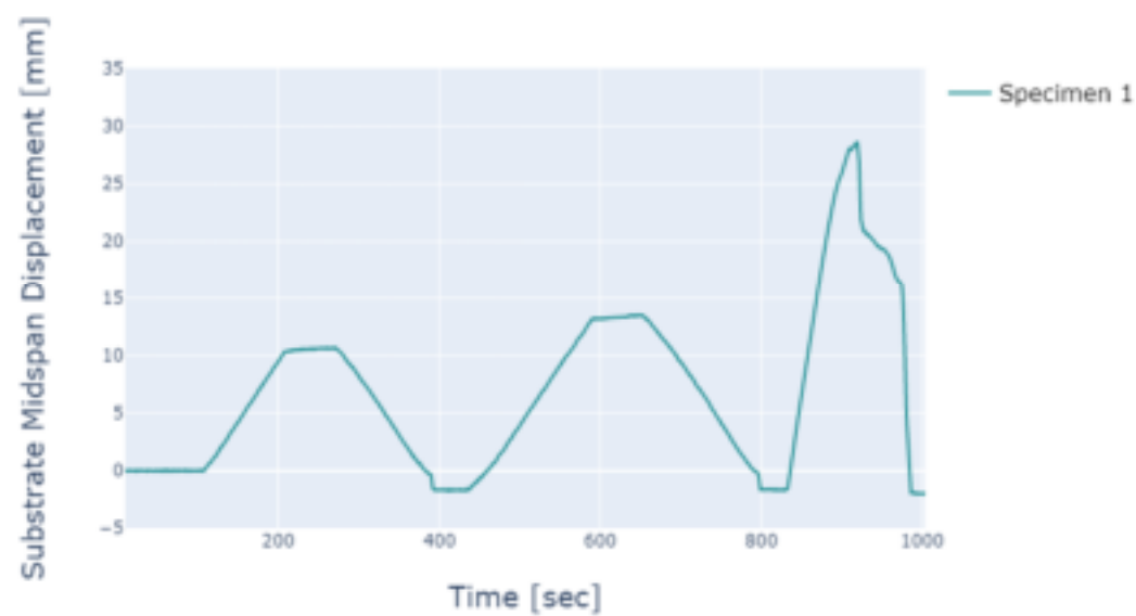
Appendix Figure C-4. ST900 specimen 1 substrate midspan displacement results
