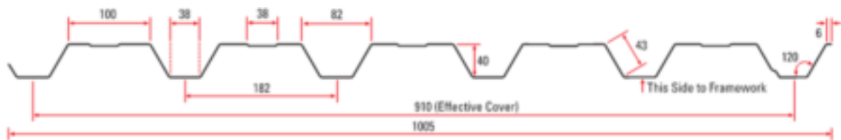
Figure 3-5. Proposed substitute: MultiRib section geometry (shown in intended orientation).
