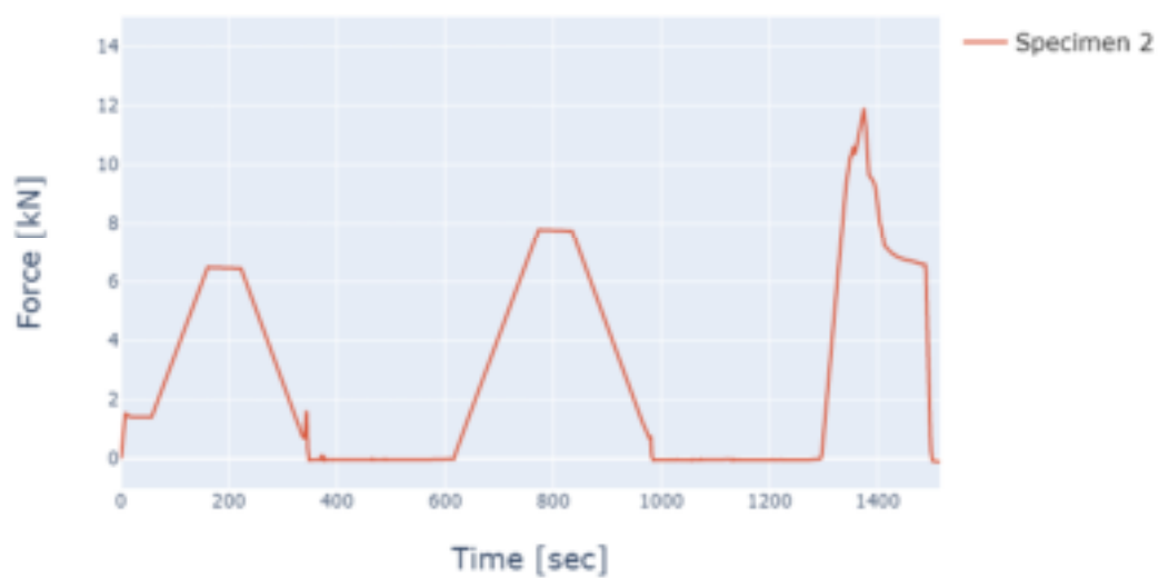
Appendix Figure C-2. ST900 specimen 2 force results
