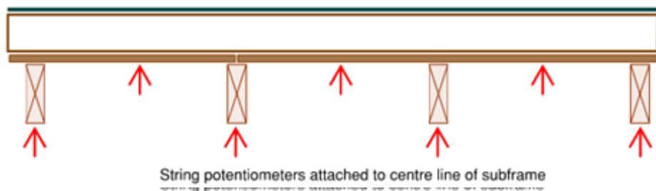
Figure 9-2. String potentiometer locations on plywood subframe during SLS tests
