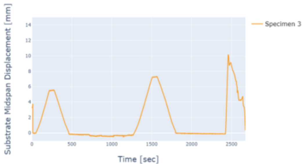
Appendix Figure B-6. Ecoply specimen 3 substrate midspan displacement results
