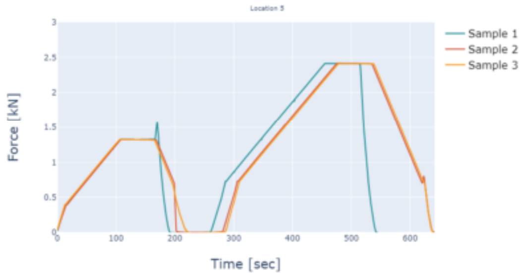
Appendix Figure A-6. Location 5 (midspan) force results
