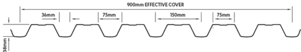
Figure 3-2. Existing ST900 profile (Note: Installed inverted as shown).
