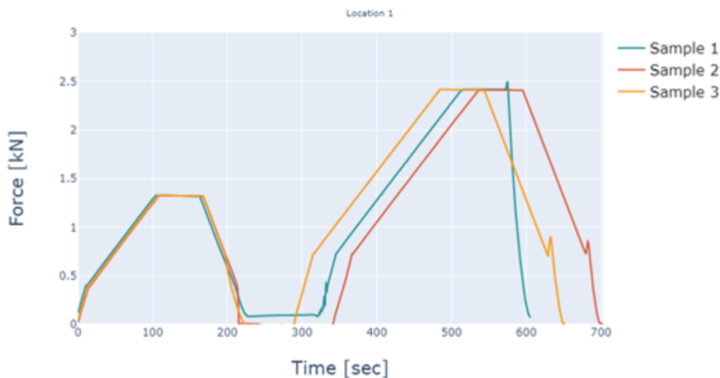
Figure 8-12. Location 1 (female side of joint) force results
