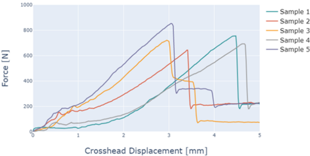
Figure 7-6. Viking Soudafoam force-displacement results
