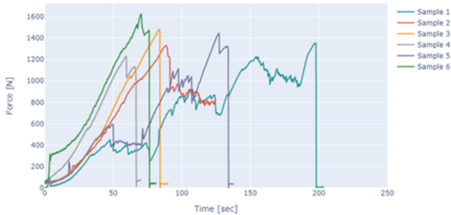
Figure 5-4. Carlisle HP-X fastener in ST900 sheeting force-displacement results
