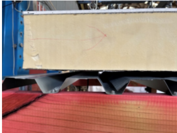
Figure 9-19. Washer pulling through PIR affixed to ST900
