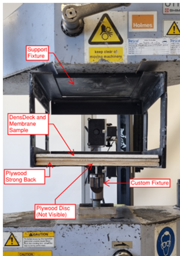
Figure 7-1. Membrane pull off test set up
