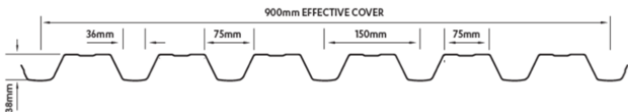
Figure 3-2. ST900 Profile (Note: Installed inverted as shown)
