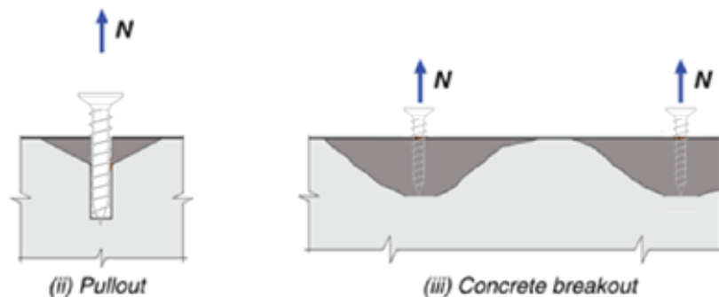
Figure 5-1. Pull Out and Break Out Failure Modes (ACI 318-19)
