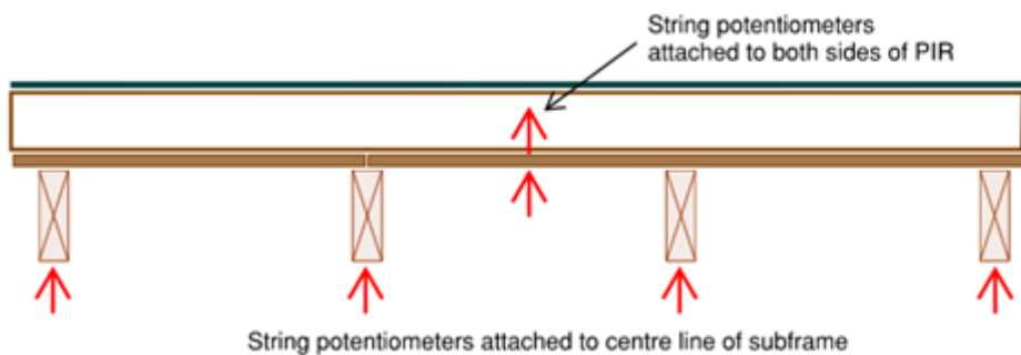
Figure 9-3. String potentiometer locations on plywood subframe during SLS tests
