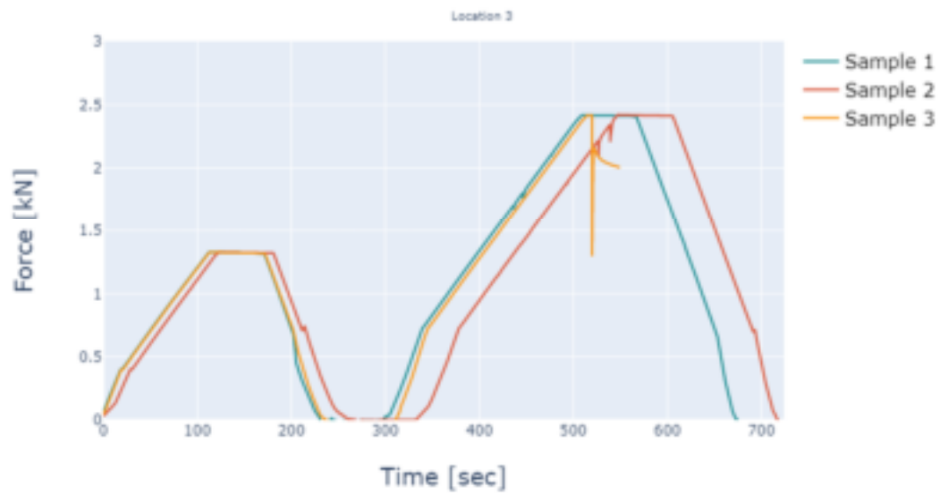
Appendix Figure A-5. Location 3 (unsupported edge) force results
