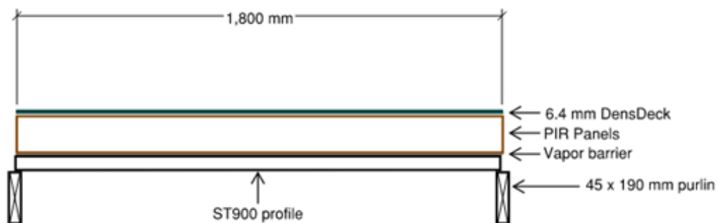
Figure 9-11. Viking Roofspec roof build up on ST900 steel roofing
