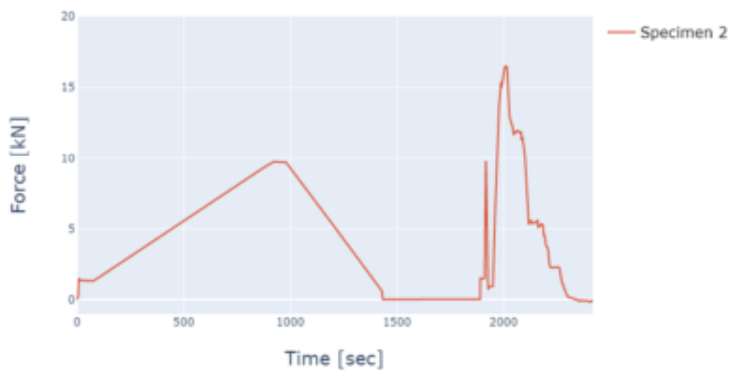
Appendix Figure B-2. Ecoply specimen 2 force results
