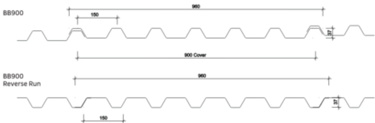
Figure 3-6. Proposed substitute: BrownBuilt 900 section geometry (lower profile shown in intended orientation).
