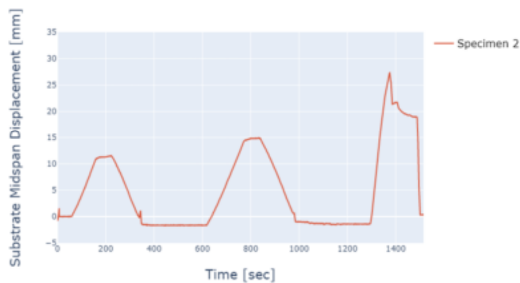
Appendix Figure C-5. ST900 specimen 2 substrate midspan displacement results
