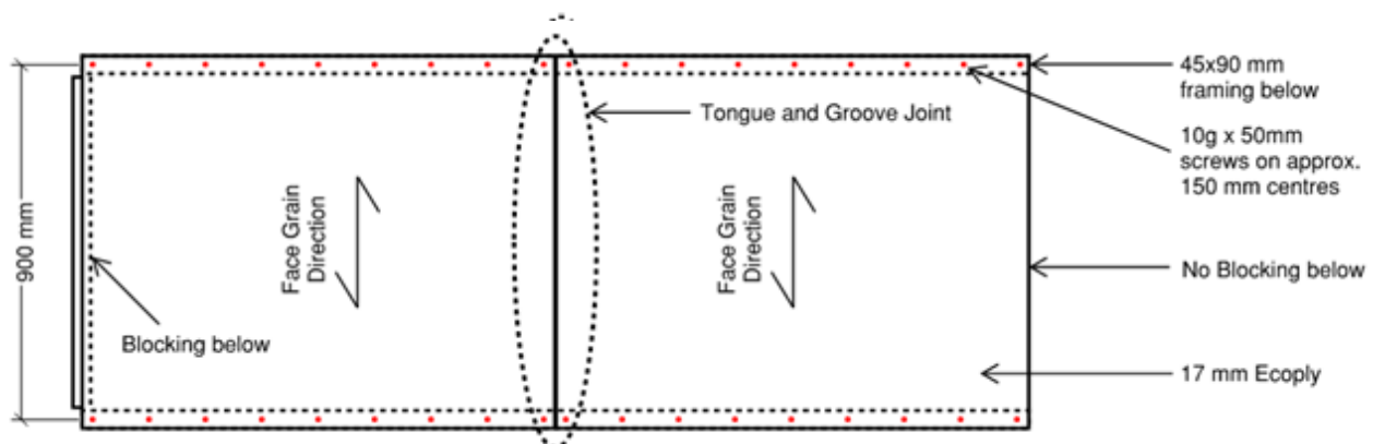
Figure 8-4. Plywood point load testing specimen
