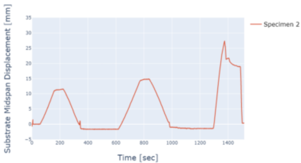
Figure 9-17. ST900 specimen 2 substrate midspan displacement results
