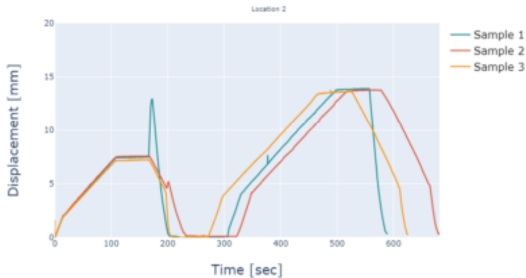
Appendix Figure A-1. Location 2 (male side of joint) displacement results
