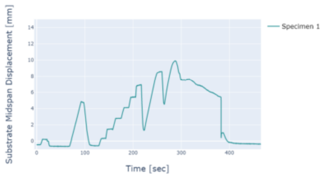
Appendix Figure B-4. Ecoply specimen 1 substrate midspan displacement results
