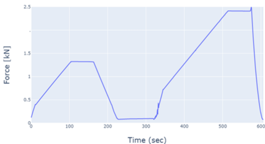
Figure 8-5. Point load testing loading protocol
