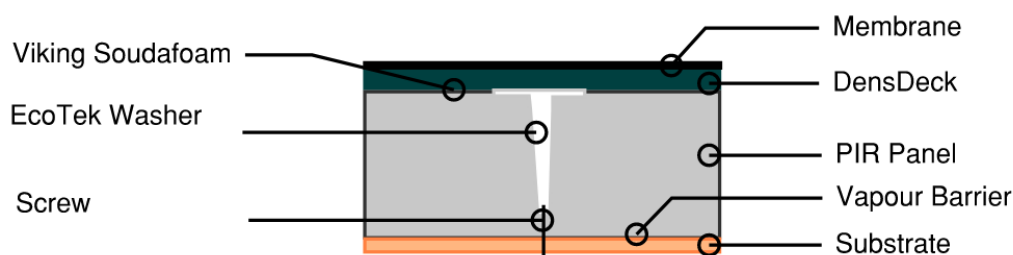
Figure 3-1. Viking RoofSpec Example Build Up
