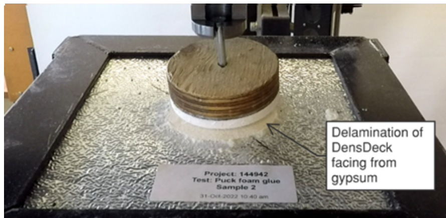
Figure 7-4. Viking Soudafoam pull off test specimen after loading
