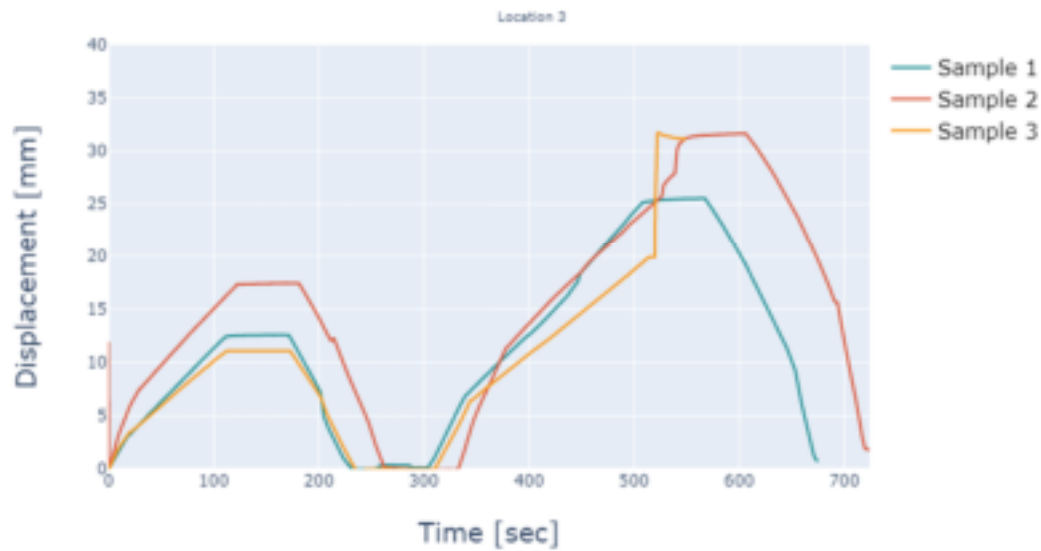
Appendix Figure A-2. Location 3 (unsupported edge) displacement results
